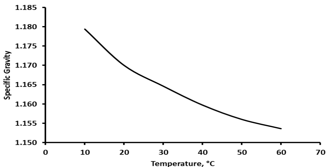
Specific Gravity as a Function of Temperature
